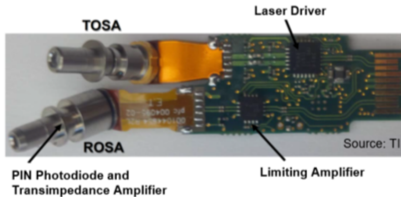
Figure 1: Optical transceiver.
