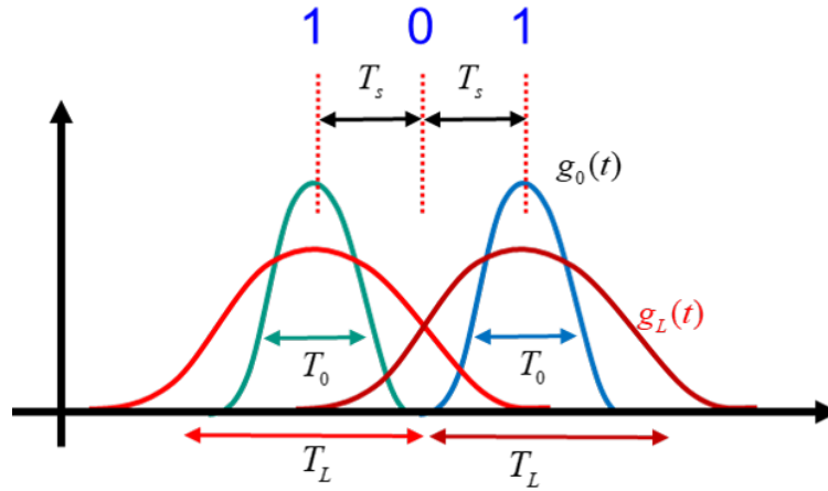
Figure 3: Sketch showing the effect of broadening of a pulse.
